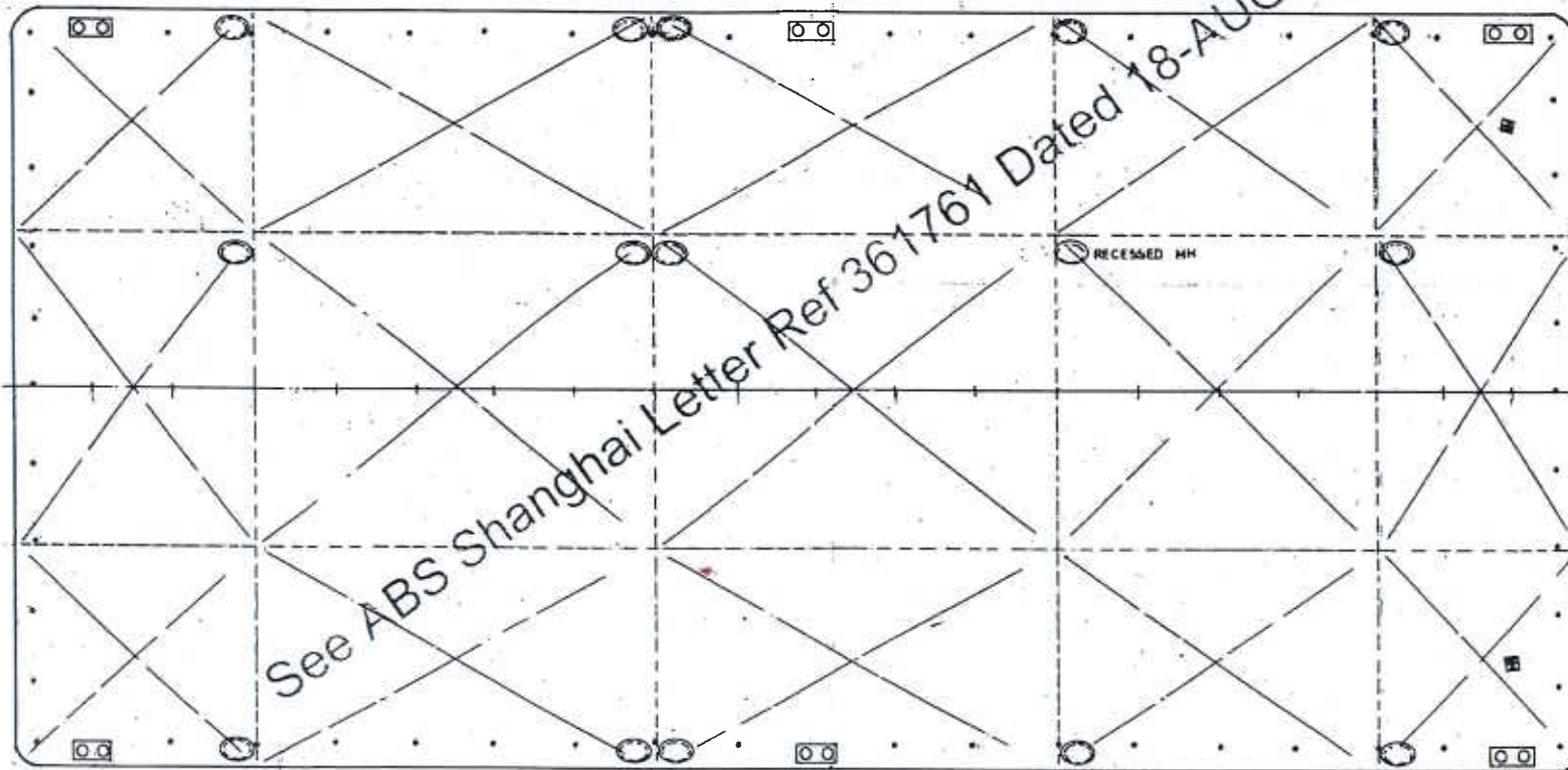
MAIN DECK
